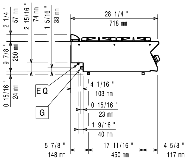
Lateral
